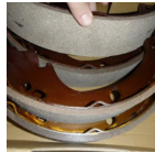
Rear and Upper Brake Shoes Sub-Assembly for Toyota Forklift
